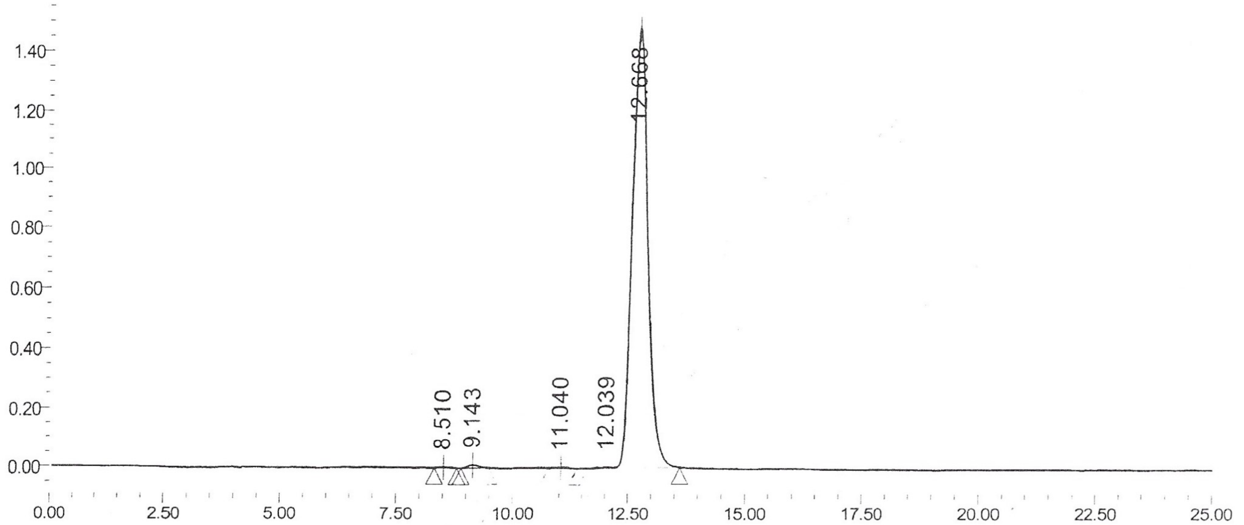
Auto-Scaled Chromatogram
